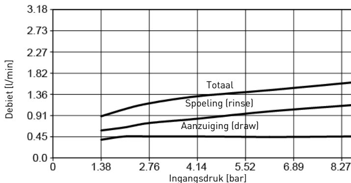
INJECTOR 00
